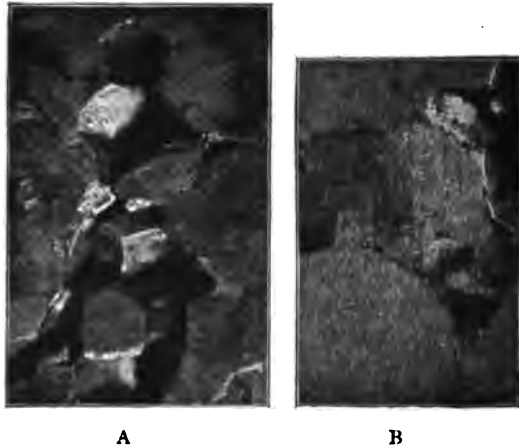
Fig. 78. Burnt Steel of 0.50 Carbon. 33 Diameters. Made by W. Campbell, Ph.D., in the Author's Laboratory.
